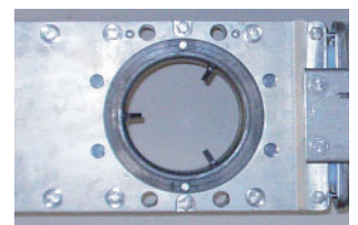
Wear minimised by conical ring with turbulence interrupter ribs
