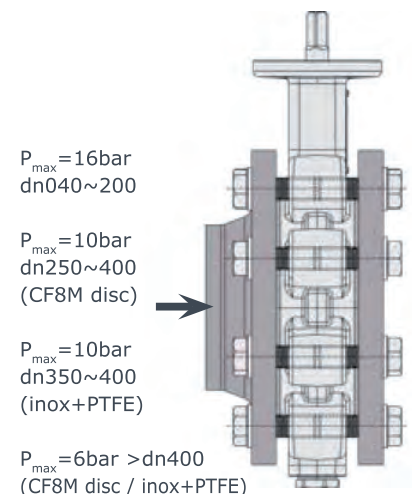
Type B installation with end piping
